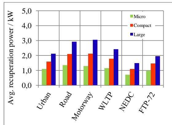
Figure 6: Average electric recuperation in drive cycle
