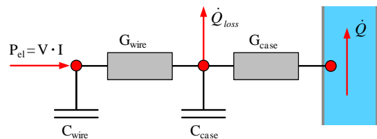
Figure 2: Electric brake resistor simulation model
