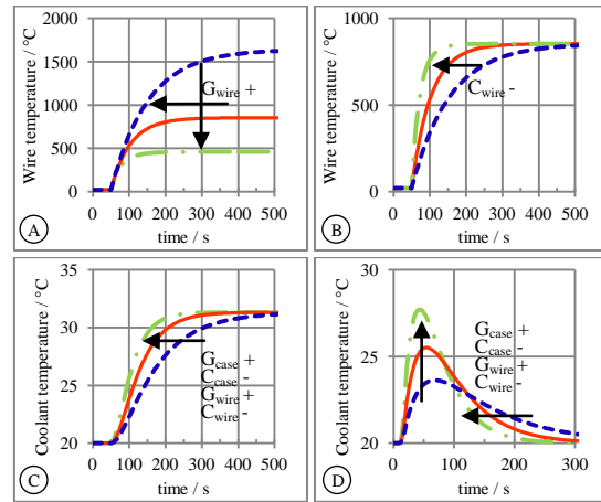
Figure 4: Impact of model parameters on thermal behavior of brake resistor
