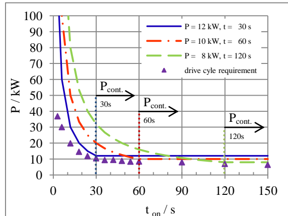
Figure 8: Exemplary comparison of brake resistor performance and drive cycle requirement
