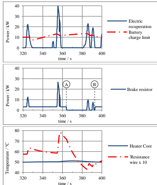
Figure 10: Visualization of brake resistor control
