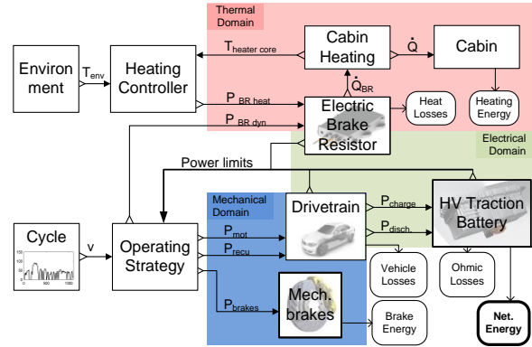
Figure 9: Schematic of simulation environment
