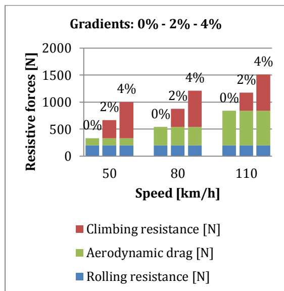
Figure 8: AGV Connect resistive force distribution for different speeds and road inclination.
