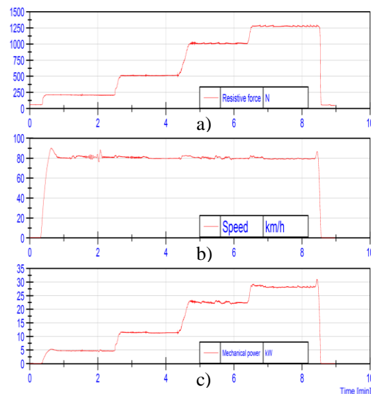
Figure 9: AGV measured a) resistive force, b) speed, c) mechanical power, during roller bench test at 80km/h.
