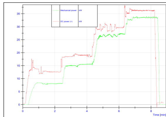
Figure 10: AGV electrical battery power (red) and mechanical wheel power (green) at 80km/h test.
