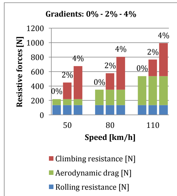
Figure 3: iOn resistive force distribution for different speeds and road inclination.
